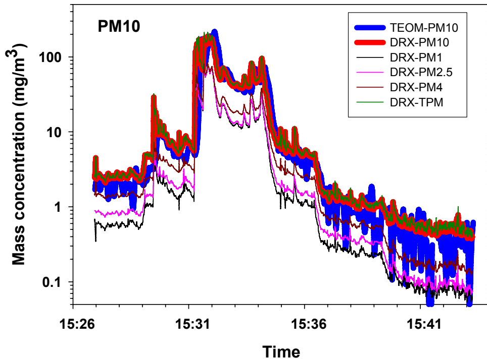
Figure 1a. Comparison of Arizona Road Dust (A1) mass concentration measured by the DUSTTRAK DRX and the TEOM with a PM 10 impactor.
