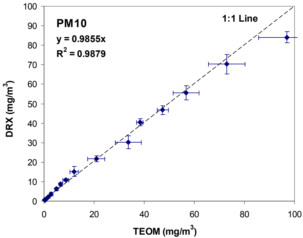
Figure 2a. Linear correlation between DUSTTRAK DRX and TEOM for Arizona Road Dust (A1) mass concentration measurement. The TEOM ran with a PM 10 impactor.
